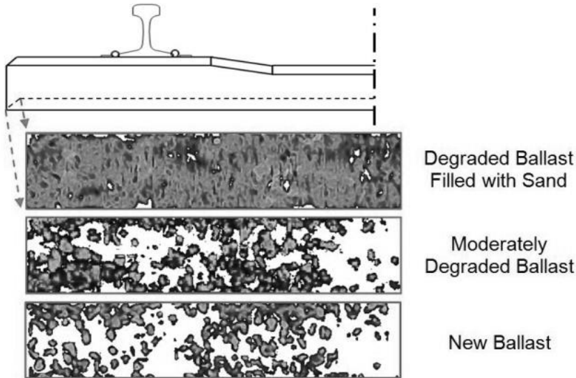
6 7 8 FIGURE 10 Three qualitative pressure distributions along the length of a test tie for three 9 different ballast gradations.
