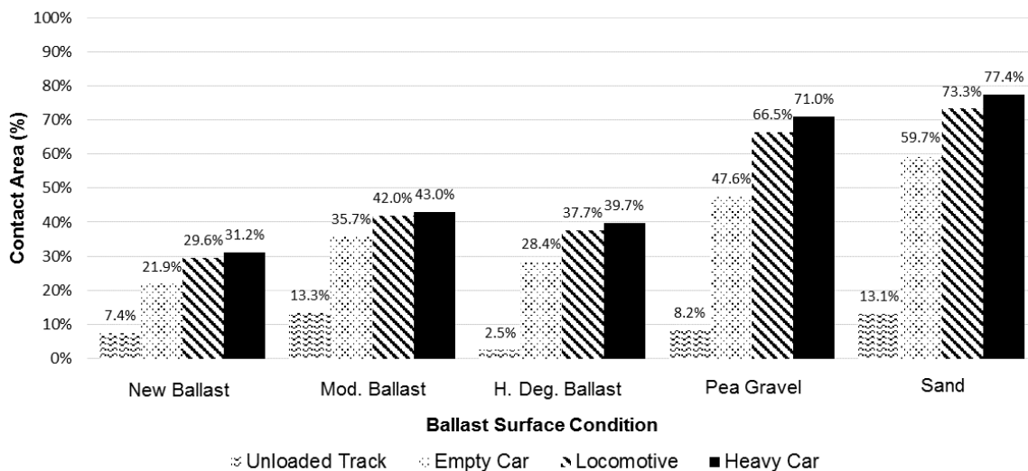
14 15 16 FIGURE 11 Average contact areas in each zone for each applied axle load. 17
