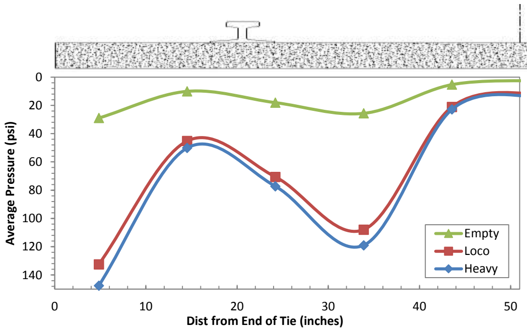
Figure 7.12 Average pressure distributions along Tie 39 for the three applied axle loads
